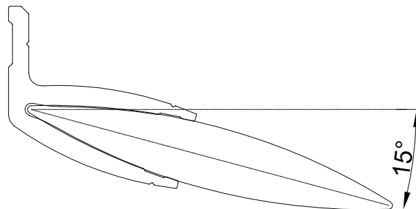
U15/ST 150
