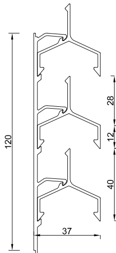
ST 40V
